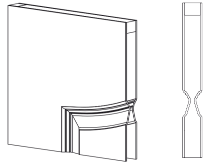
Cove & Bead Sticking
