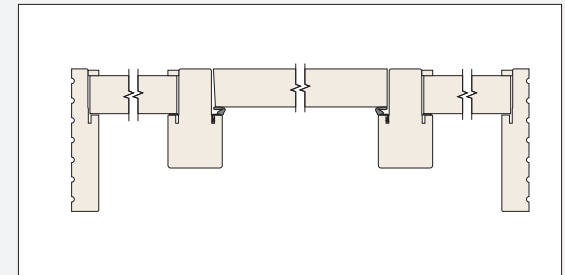
Single Rabbet Frame with 4 9/16" Uniframe Mull Posts
