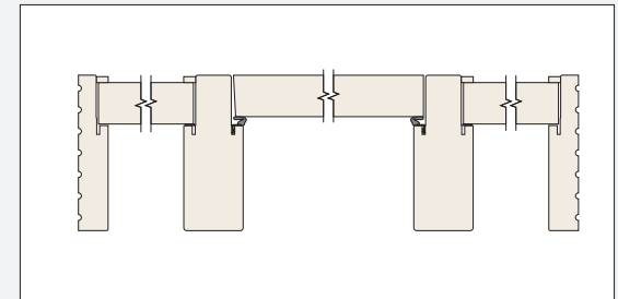
Single Rabbet Frame with 6 - 9/16" Uniframe Mull Posts
