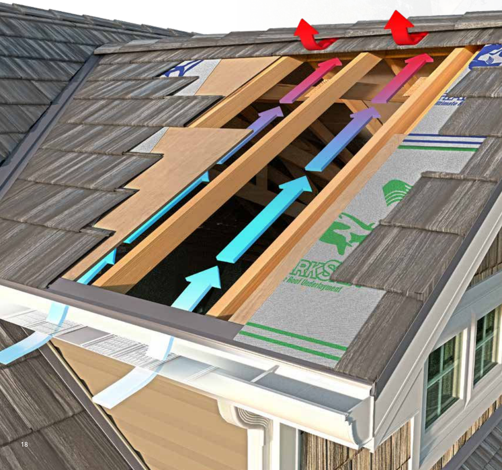
Underlayment
