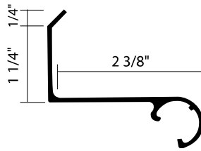
2 - 3/8" Female Hinge
