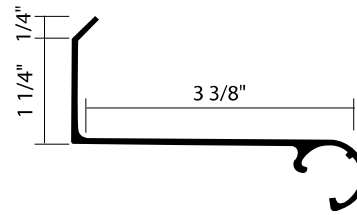
3 - 3/8" Female Hinge
